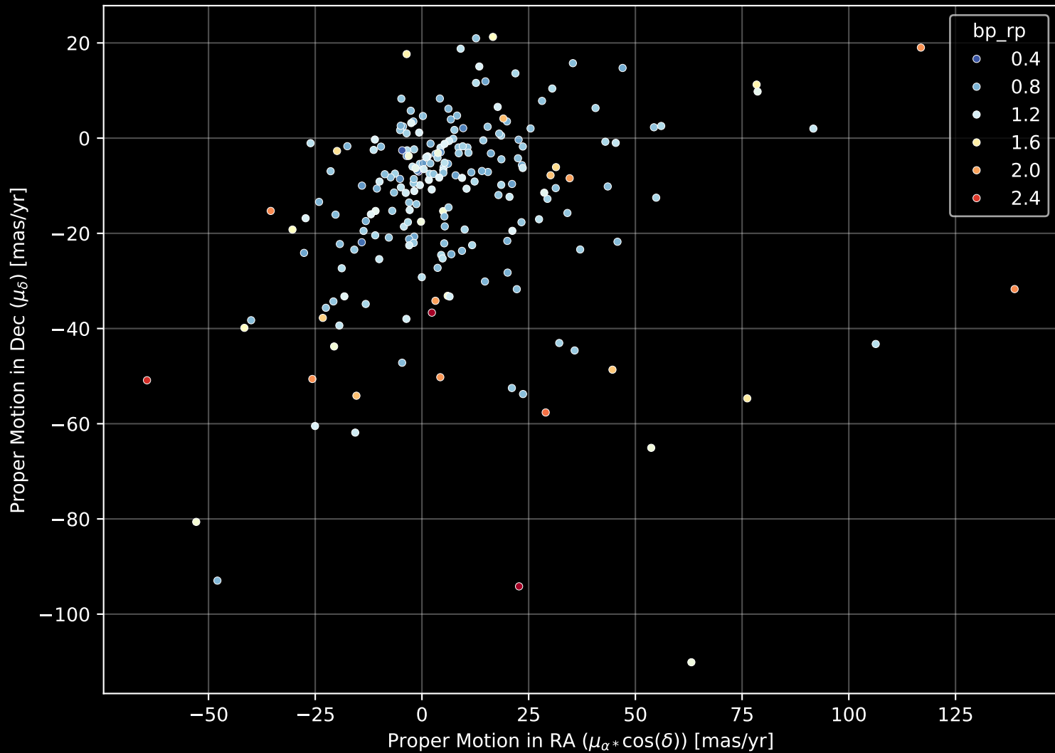
APOGEE DR17 Field: [056-50-O] Proper Motion Diagram (n= 217)
