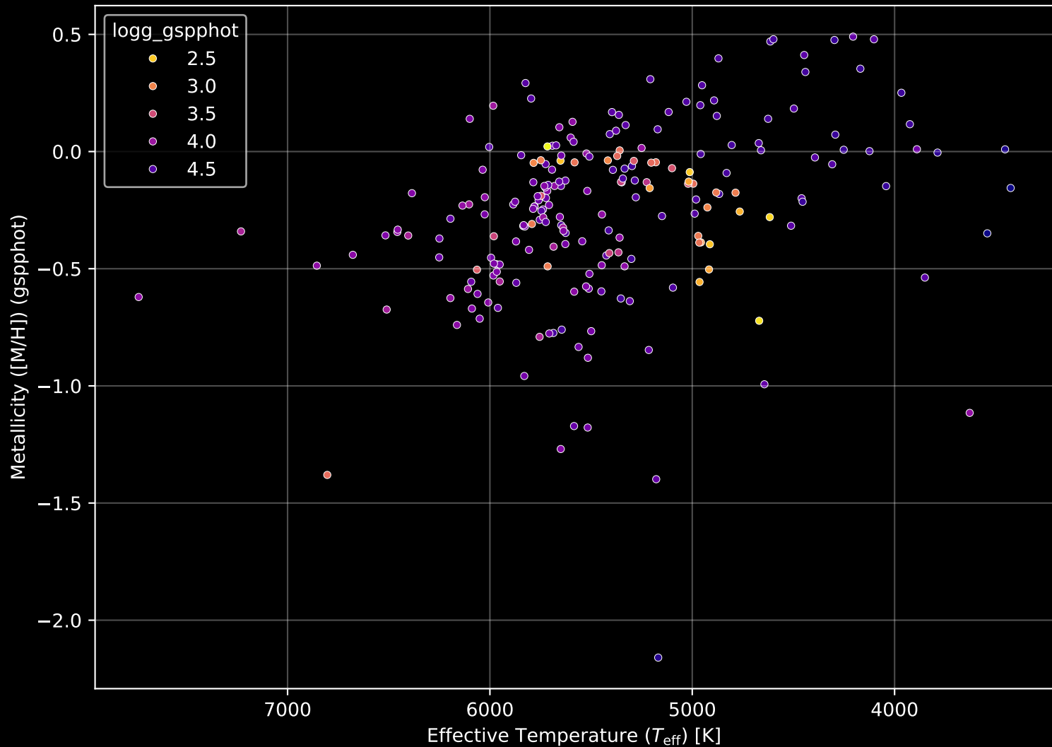
APOGEE DR17 Field: [056-50-O] Stellar Population Parameters (n= 217)
