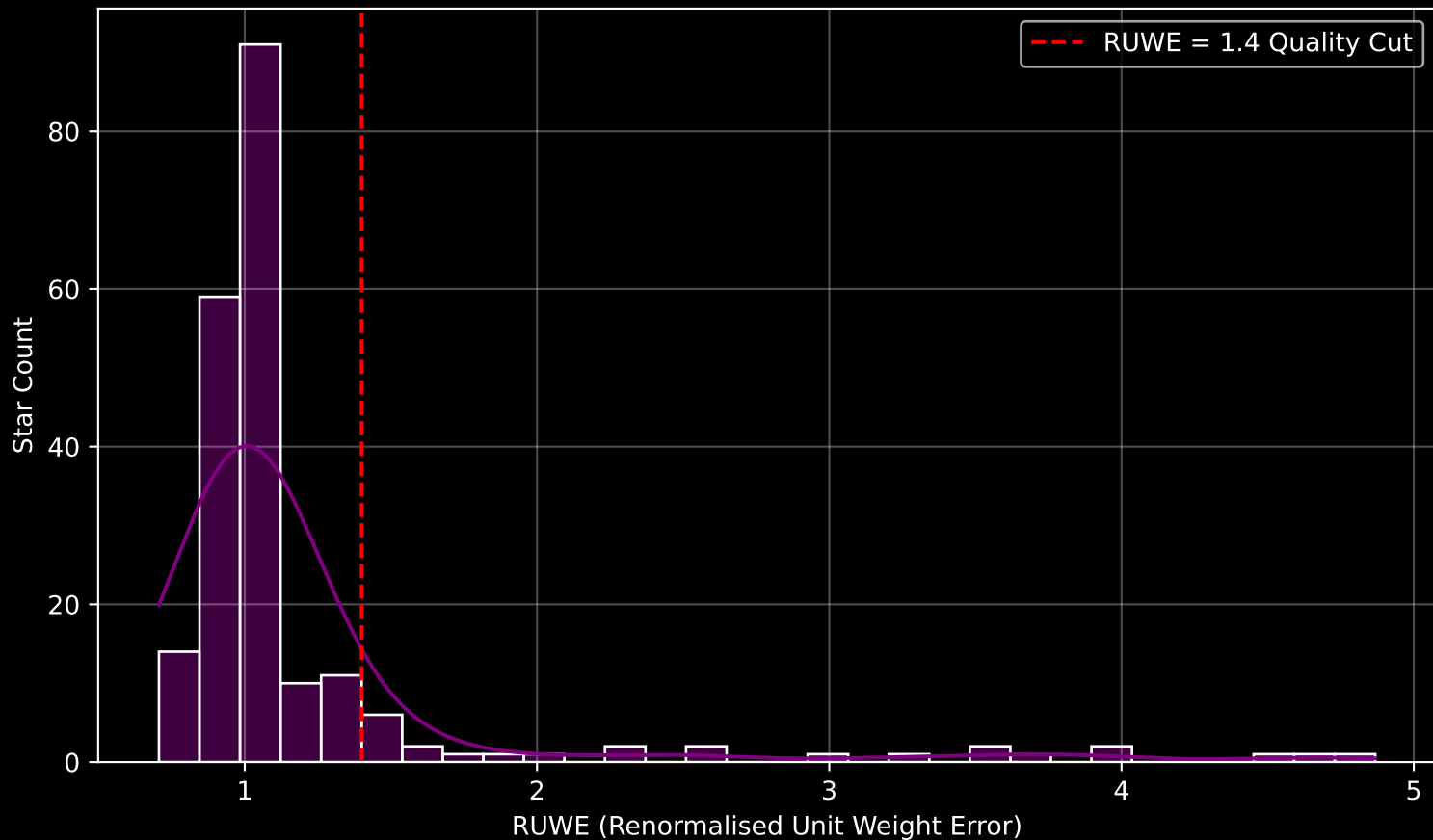
GAPOGEE DR17 Field [056-50-O] RUWE Distribution (n= 210)
