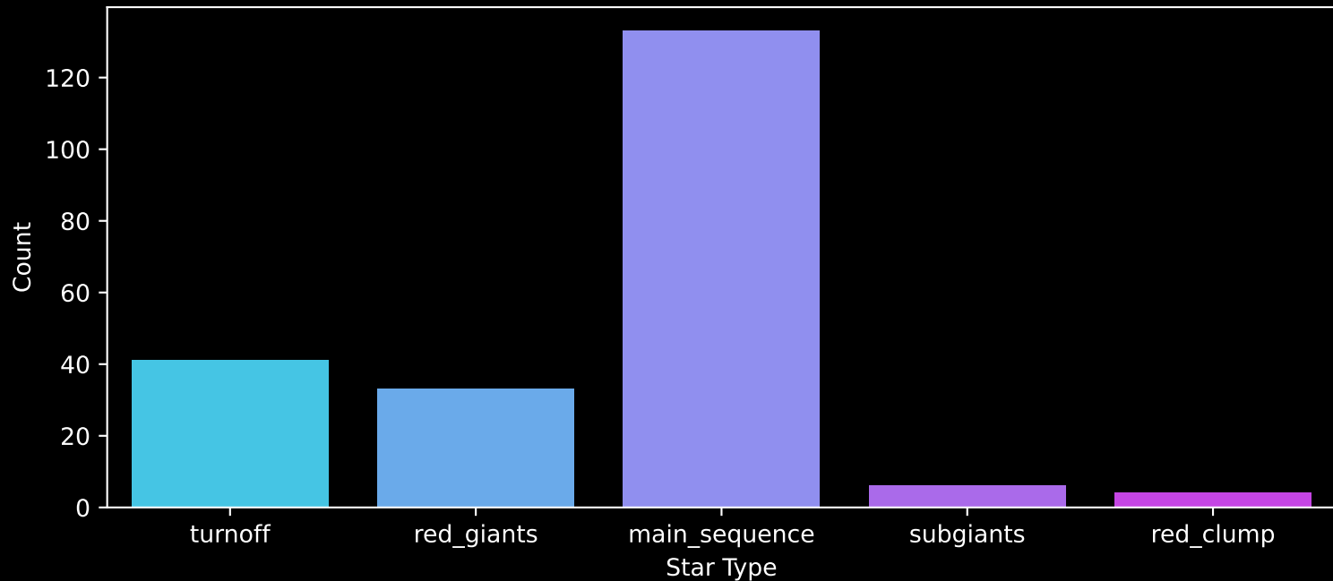
APOGEE DR17 Field: [056-50-O] Count plot of Star Type
