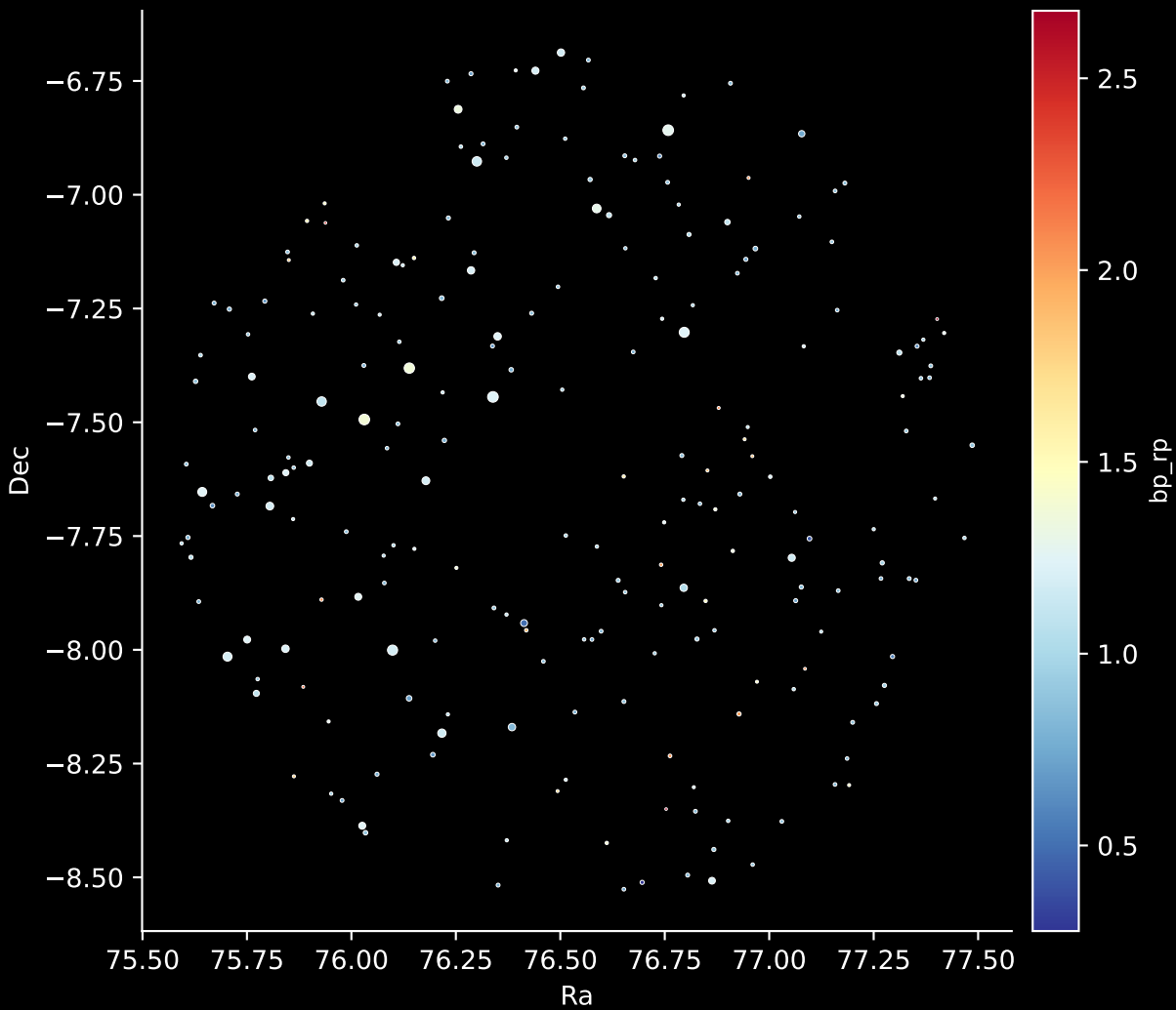
APOGEE DR17 Field: [056-50-O] Stars: 217
