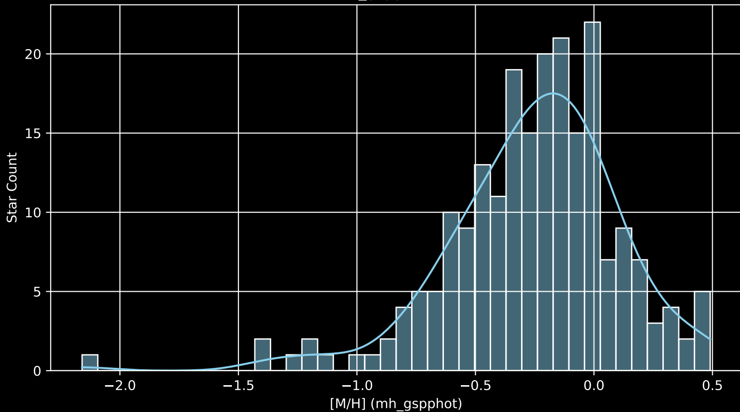
APOGEE DR17 Field: [056-50-O [M/H] (mh_gspphot) (n= 217)
