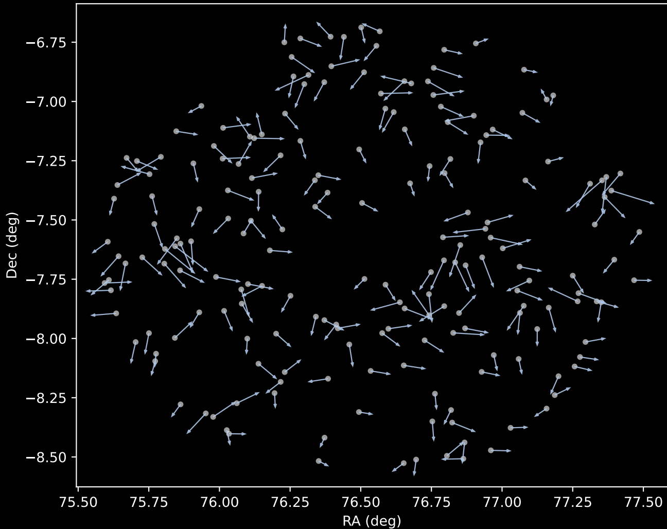
APOGEE DR17 Cluster 1 Proper Motion Vectors (n=195)
