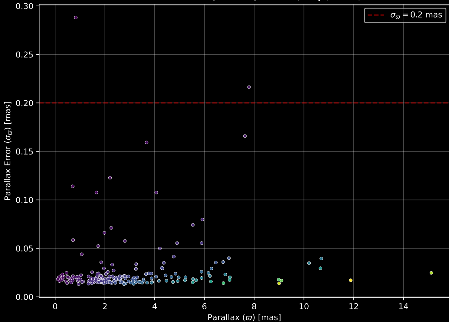
APOGEE DR17 Field: [056-50-O] Parallax Quality (n= 217)
