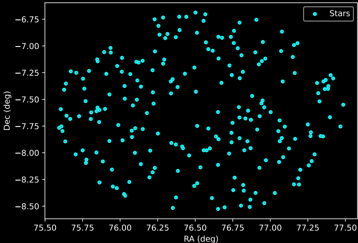
APOGEE DR17 Field: [056-50-O] Proper Motion Vectors for Gaia Star Field (n= 217)
